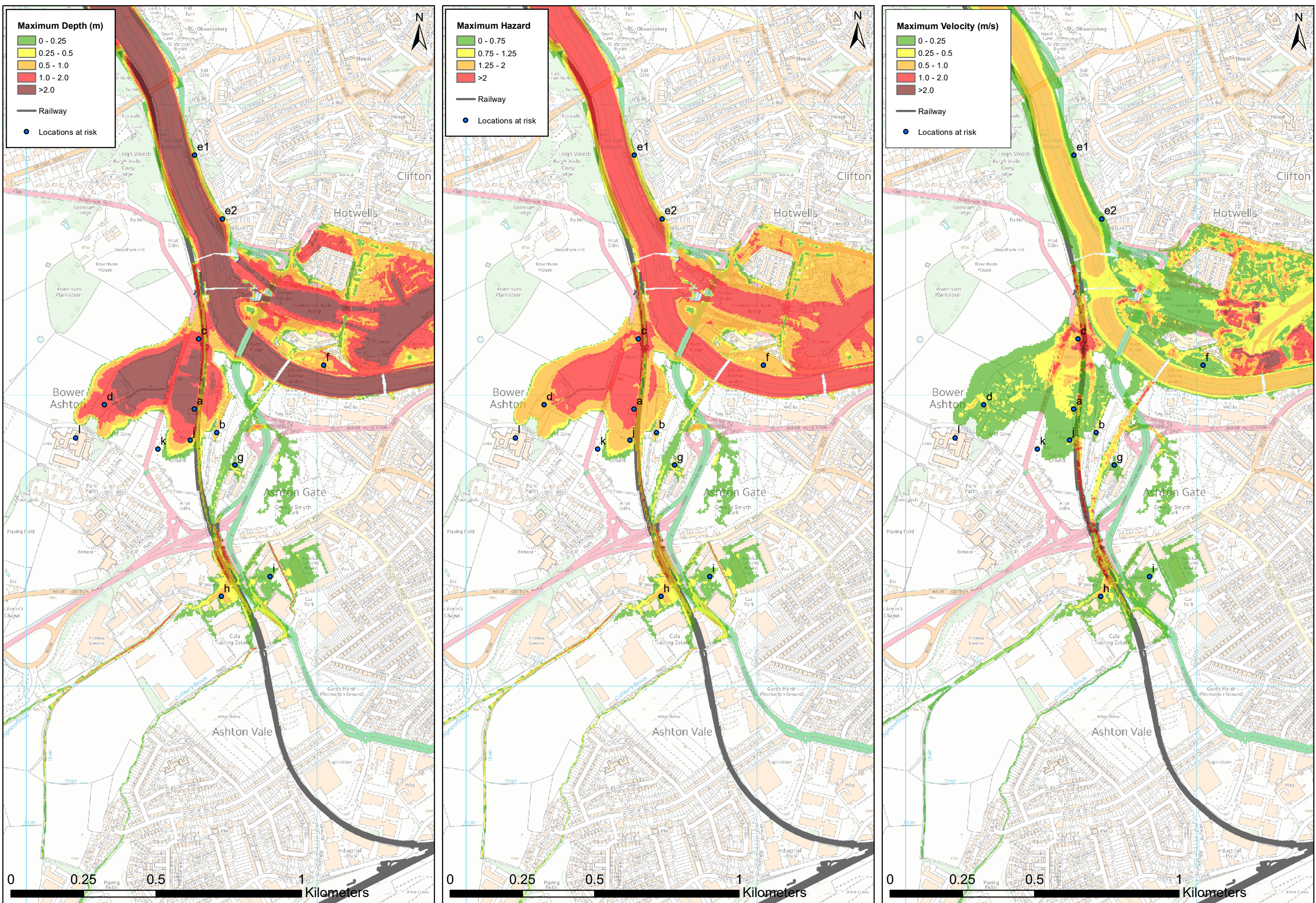
Figure N-26: Post Development, 75year return period event in 2115 ,Tidal
